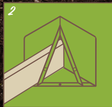
2 SLIDE BOARD DOWN INTO BRACE, FLUSH WITH THE CORNER OF THE BRACE
