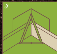
3 SLIDE SECOND BOARD DOWN INTO BRACE, FLUSH WITH THE FIRST BOARD AND THE SIDE OF THE BRACE
